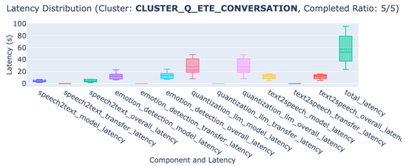
Figure 6: Screenshot of the end-to-end latency benchmark statistics for the setup: Local Whisper , Emotion Detection , Quantization LLM , and OpenAI Text-to-Speech . This visualization is one example of the generated benchmark report; you can customize it or explore more details within our demo.
